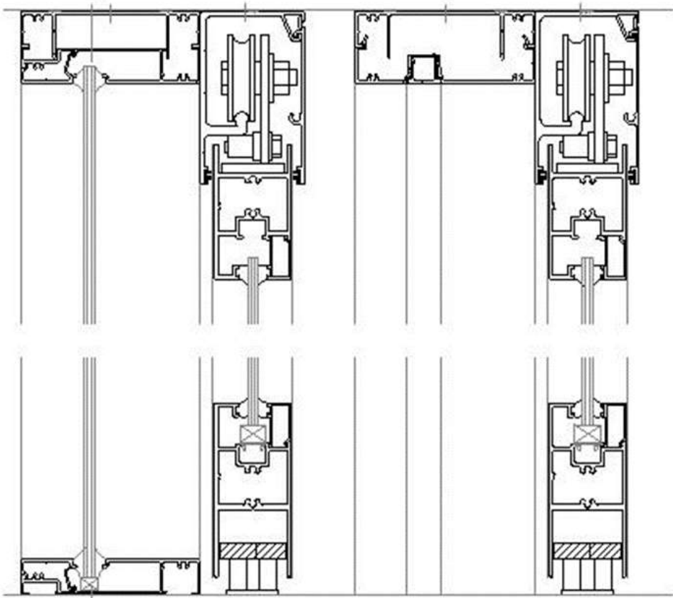
Full Height Glazing Frame
