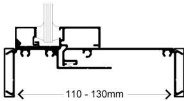
Adjustable Glazing Frame Kits
