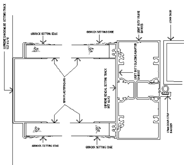
07 SECTION 'F' LIGHT DUTY SHOPFRONT & SUPREME 64 SETTING 13/07/2008
